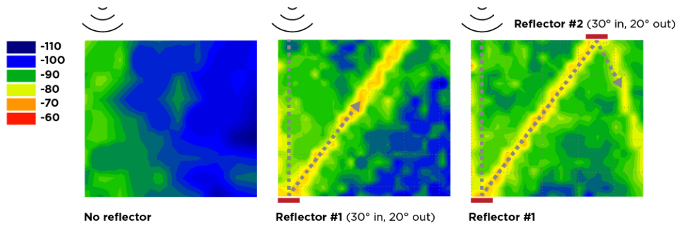
Figure 15: Use case of Reflection deployment
