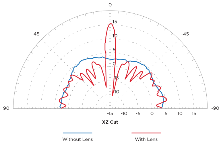
Figure 16: Radiation pattern before and after applied Enhancement lens
