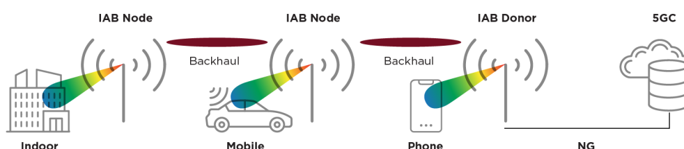
Figure 12: Reference IAB Diagram System and Application Architecture (refer to 3GPP TR 38.874)
